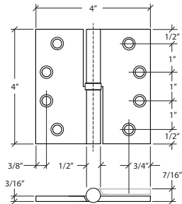
29738L OR 29738R 4" X 4" LIFT OFF HINGE ROUND BARREL - BALL BEARING SPECIFY LEFT OR RIGHT HAND
