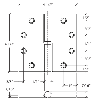
29739L OR 29739R SPECIFY LEFT OR RIGHT HAND 4-1/2" X 4-1/2" LIFT OFF HINGE ROUND BARREL - BALL BEARING SPECIFY LEFT OR RIGHT HAND
