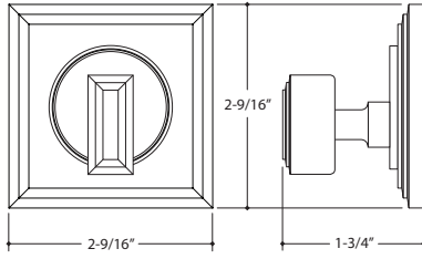
20041_T DEADBOLT COLLAR 22010 THUMB TURN
