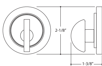
20057_T DEADBOLT COLLAR 22060 THUMB TURN
