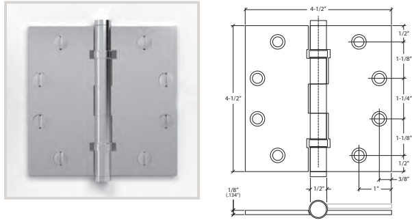
29640 4-1/2" X 4-1/2" BALL BEARING HINGE SQUARE CORNERS
