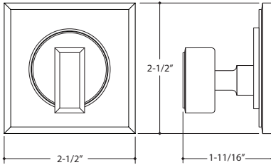
20072_T DEADBOLT COLLAR 22011 THUMB TURN
