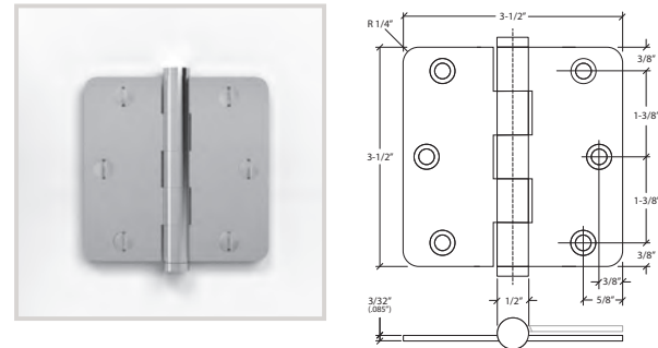
29560 3-1/2" X 3-1/2" RESIDENTIAL HINGE 1/4" RADIUS CORNERS
