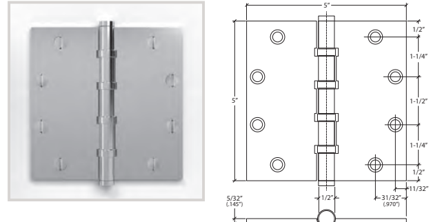
29651 5" X 5" BALL BEARING HINGE SQUARE CORNERS
