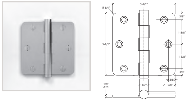
29550 3-1/2" X 3-1/2" ARCHITECTURAL HINGE 1/4" RADIUS CORNERS
