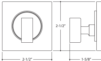
20051_T DEADBOLT COLLAR PRE-BORED DOOR 22009 THUMB TURN
