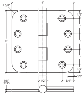
29610 4" X 4" ARCHITECTURAL HINGE 5/8" RADIUS CORNERS
