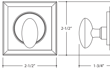
20347_T DEADBOLT COLLAR 22004 THUMB TURN (SHOWN)
