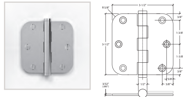
29580 3-1/2" X 3-1/2" RESIDENTIAL HINGE 5/8" RADIUS CORNERS
