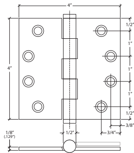
29590 4" X 4" ARCHITECTURAL HINGE SQUARE CORNERS
