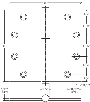
29650 5" X 5" ARCHITECTURAL HINGE SQUARE CORNERS
