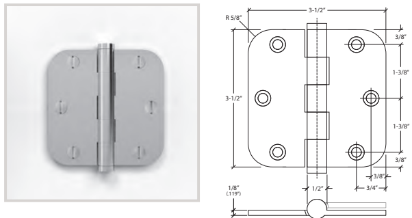
29570 3-1/2" X 3-1/2" ARCHITECTURAL HINGE 5/8" RADIUS CORNERS
