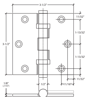
29530 3-1/2" X 3-1/2" BALL BEARING HINGE SQUARE CORNERS
