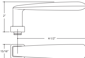
23024 DOOR LEVER Pricing Tier I Levers are broached 8mm on the square and drilled for left or right hand.
