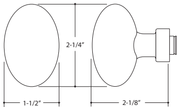
25011 DOOR KNOB Hudson Collection Pricing Tier I Hand hammering available - upcharges apply.
