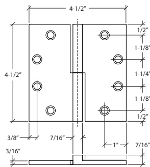
29717L OR 29717R 4-1/2" X 4-1/2" LIFT OFF HINGE SPECIFY LEFT OR RIGHT HAND
