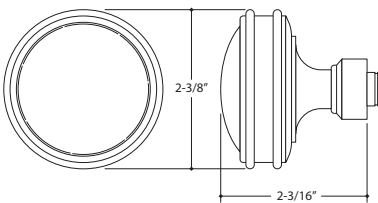
25015 DOOR KNOB Port Royal Collection Pricing Tier I Hand hammering or custom engraving available - upcharges apply.
