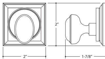
20369_T DEADBOLT COLLAR 22000 THUMB TURN
