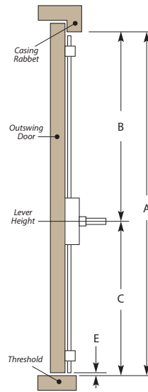
OUTSWING DOOR WITH CASING RABBET
