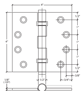
29600 4" X 4" BALL BEARING HINGE SQUARE CORNERS
