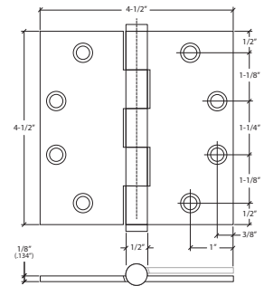
29630 4-1/2" X 4-1/2" ARCHITECTURAL HINGE SQUARE CORNERS
