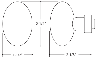
25011 OVAL DOOR KNOB Pricing Tier I
