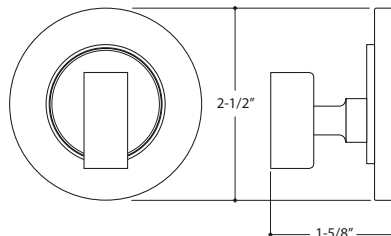
20058_T DEADBOLT COLLAR PRE-BORED DOOR 22009 THUMB TURN
