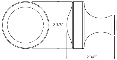
25026 DOOR KNOB Pricing Tier I Hand hammering available - upcharges apply.
