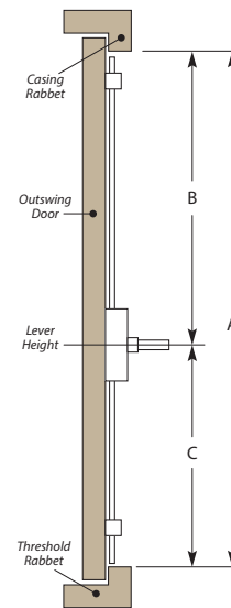
OUTSWING DOOR WITH CASING AND THRESHOLD RABBETS
